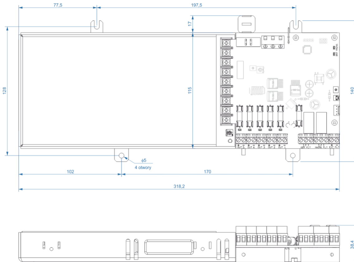
Arrangement of mounting holes and external dimensions of the ZSPM-200 and ZSPM-320 power supplies.
